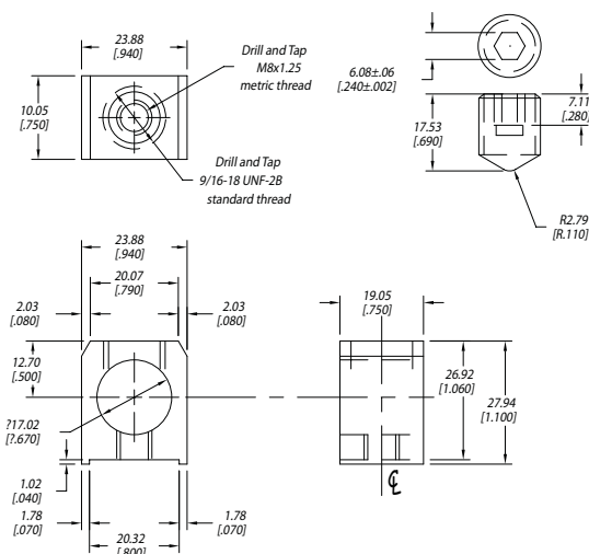
CDTL206 — for use with 200A switches
