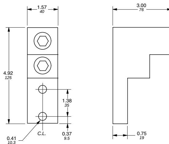
BDTL30 — for use with 800A switches
