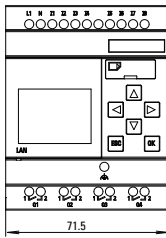
Base Module (with Display)
