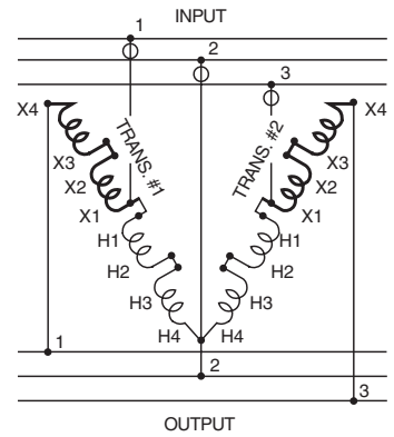
OPEN DELTA
