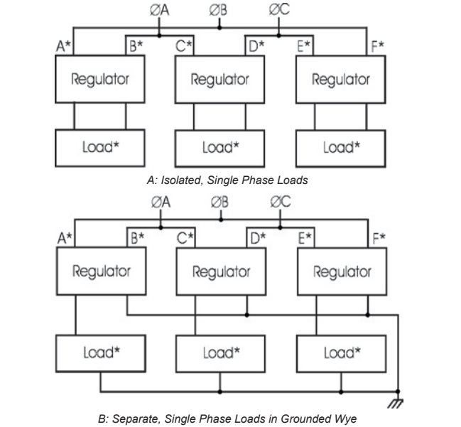
Figure 4. Three Phase Connections
