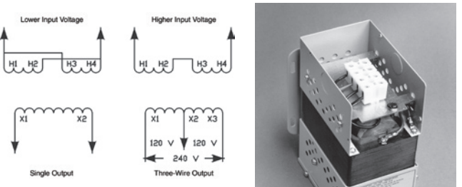
Figure 3: Electrical Connections for Non-8 models
