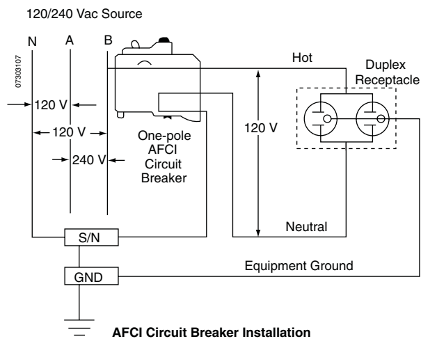
Figure 4: Typical AFCI Circuit Breaker Installation
