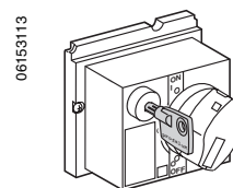
Locking of the Rotary Handle Using a Keylock
