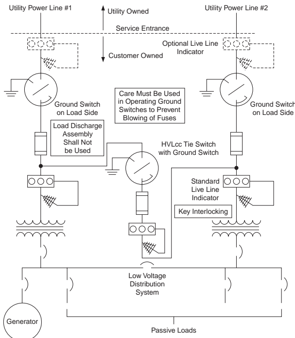
NEC Service Entrance to Double Ended Substation with or without Down Stream Generators with Fused Tie Switch Application 5
