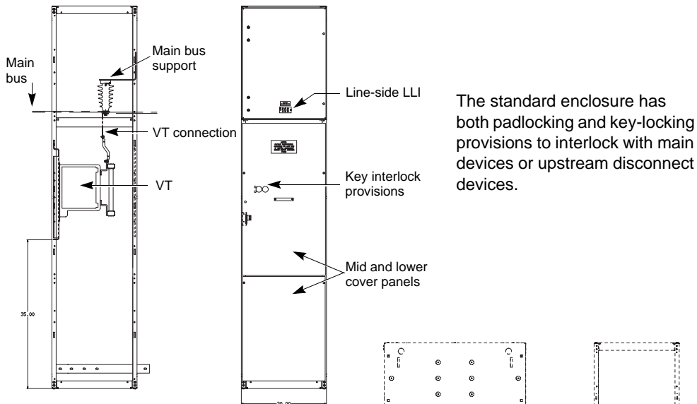
VT Section without Switch Disconnect
