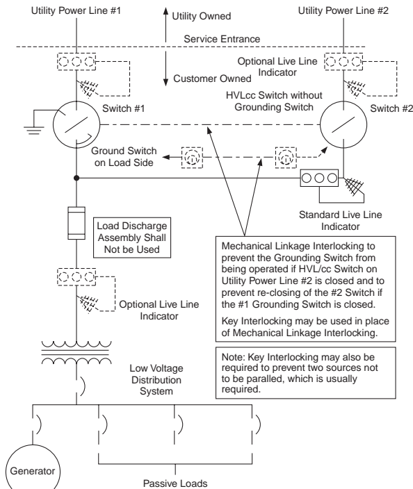
NEC Service Entrance to Duplex with Generator Loads Application 7
