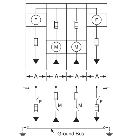
Main-Main Center Application B Located with Feeders (Application A) on Each Side (with Bottom Cable Entry and Exit)
