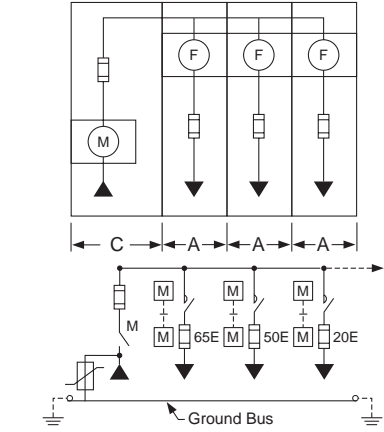
Application B Main Switch with Surge Arresters and Feeders (Bottom Cable Entry and Exit)
