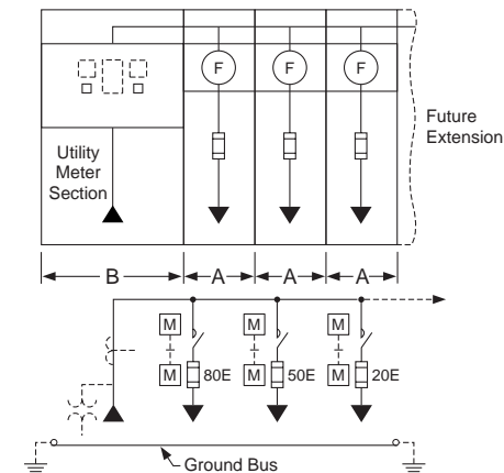
Incoming Line Hot Sequence Meter Section with Bottom Cable Entry and Exit (Feeder Line-up Application A)
