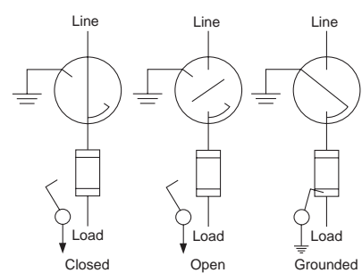
Figure 4: HVL/cc with Grounding Switch on Load Side and Load Discharge Assembly
