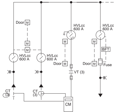
Bottom Cable Entry and Exit
