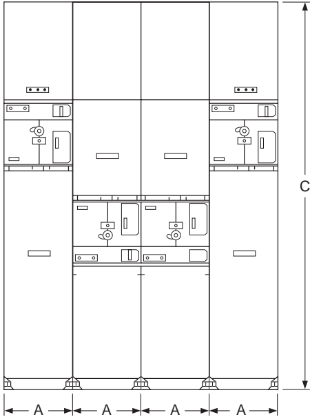
Main Switches on Ends with Feeder Switches in Center
