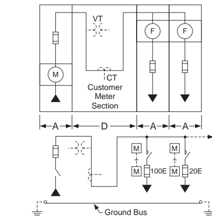
Application B Main Switch with Cold Sequence Meter Section and Two Feeder Switches Application A (with Bottom Cable Entry and Exit)
