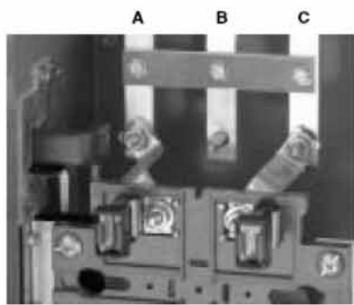
STARTING POSITION Meter Socket Phasing: AØ and CØ
