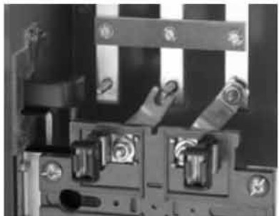
Step 3: Rotate "Z" connector to right and align with stud on BØ vertical bus.
