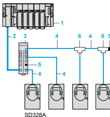
Connection via connection modules and RJ45 connectors (1)
