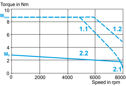
With LXM 05●D22N4 servo drive 400/480 V three-phase
