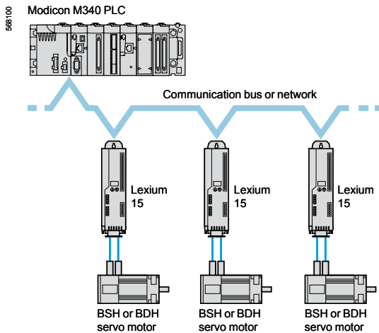
Example architecture
