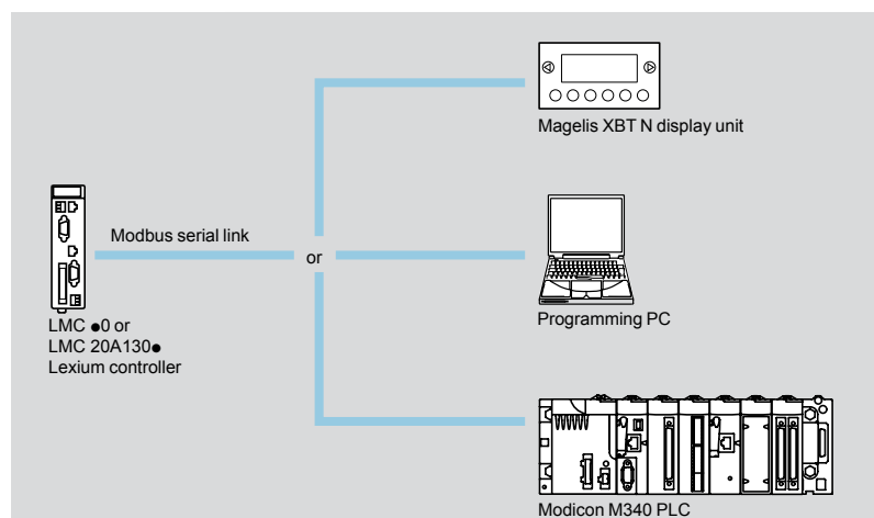
Example of architecture with Modbus serial link
