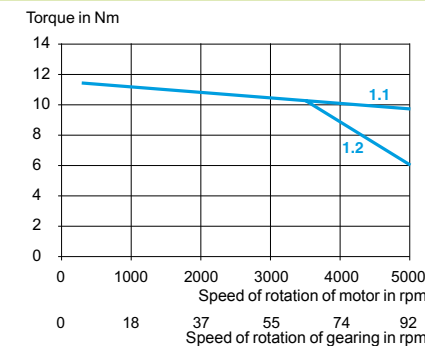
ILE1●661 with straight teeth gear G4
