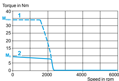
With LXM 15MD40N4 servo drive 230 V 3-phase
