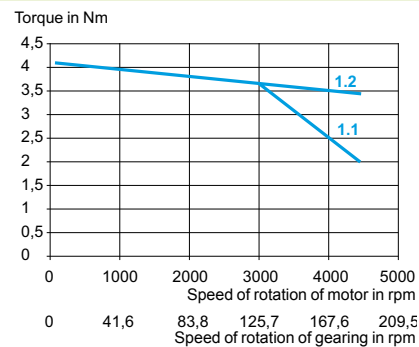
ILE2●661 with worm gear G6
