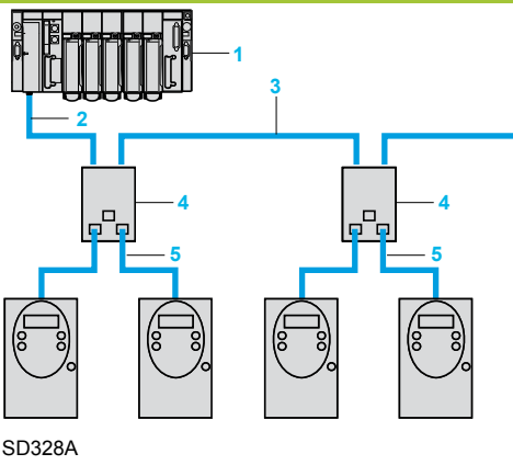
CANopen connection with junction box
