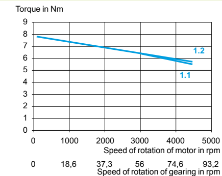
ILE1●661 with worm gear G7
