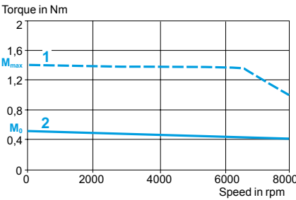
With LXM 05●D10M2 servo drive 230 V single-phase
