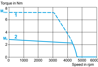
With LXM 05●D17M3X servo drive 230 V 3-phase
