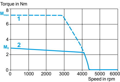
With LXM 05●D17M2 servo drive 230 V single-phase
