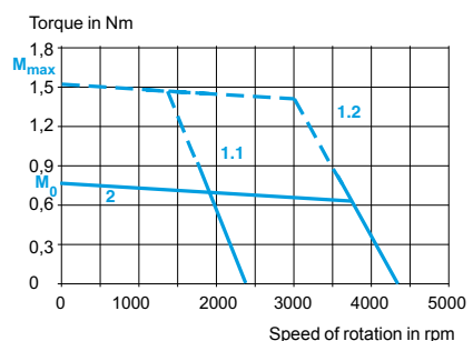
ILA2●572P (winding type P)
