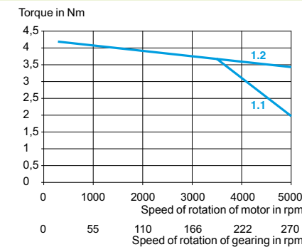
ILE1●661 with straight teeth gear G2
