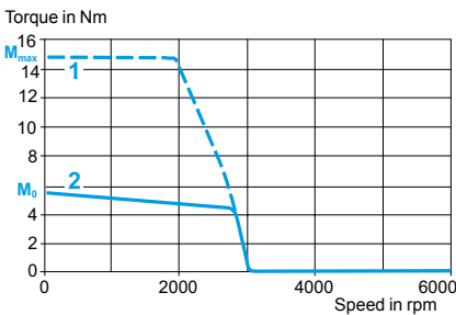
230 V 3-phase
