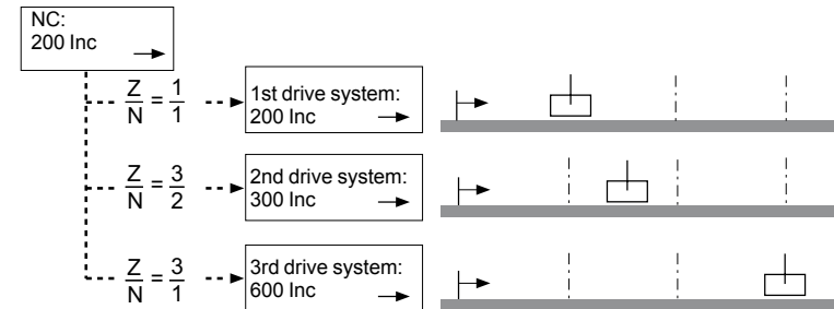
“Electronic gear” operating mode
