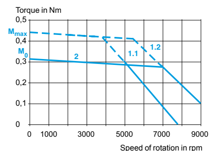
ILA2●572T (winding type T)
