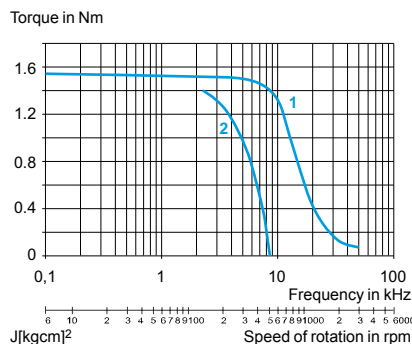
BRS368
