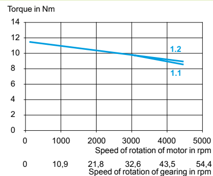
ILE2●661 with worm gear G8
