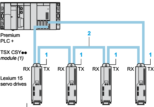
SERCOS ring network
