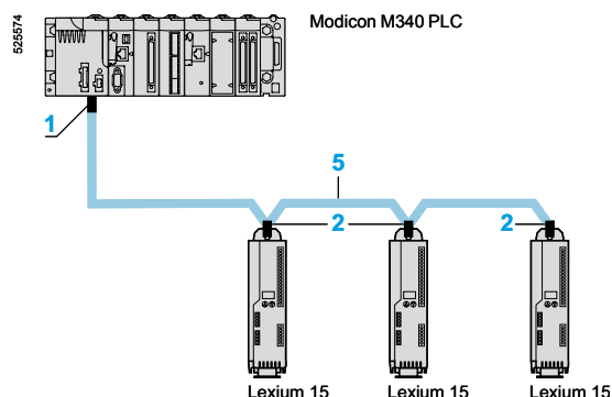
Example of connection to the CANopen machine bus with a Modicon M340 PLC
