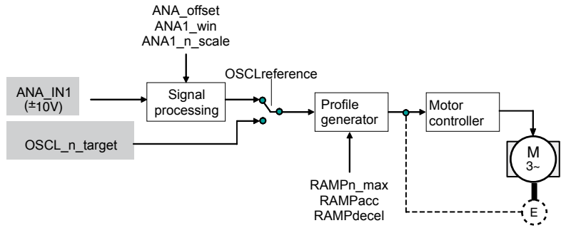
Overview of “Oscillator” operating mode
