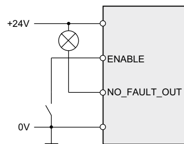
Logic type (Sink)
