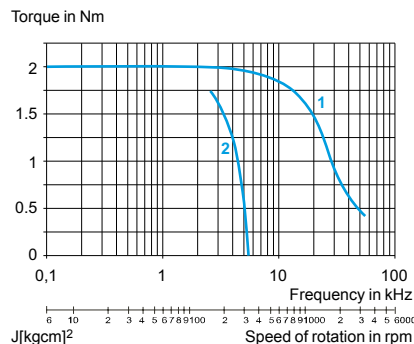
BRS397
