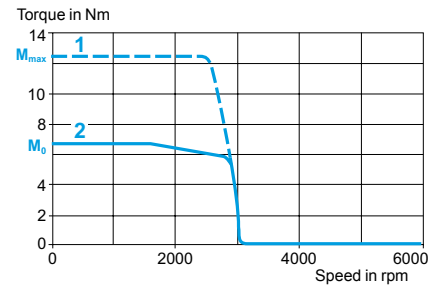
With LXM 15LD17N4 servo drive 230 V 3-phase
