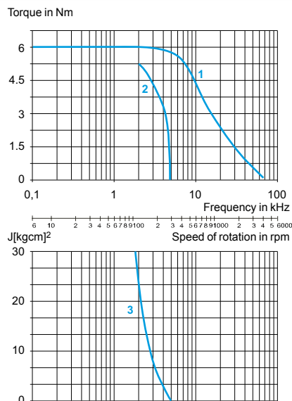
BRS39B
