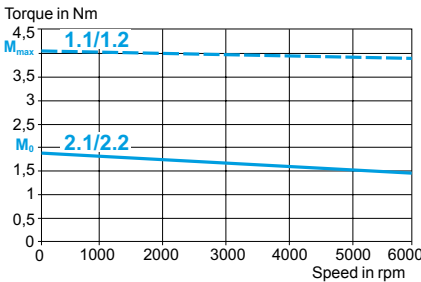
With LXM 05●D14N4 servo drive 400/480 V 3-phase
