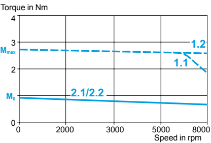
With LXM 05D14N4 servo drive 400/480 V three-phase
