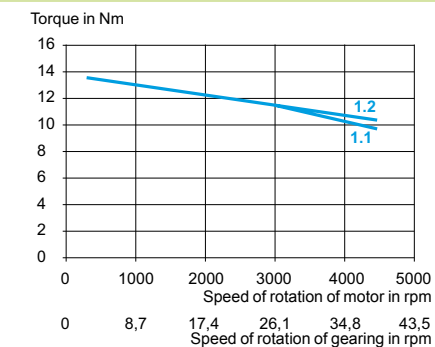
ILE1●661 with worm gear G8
