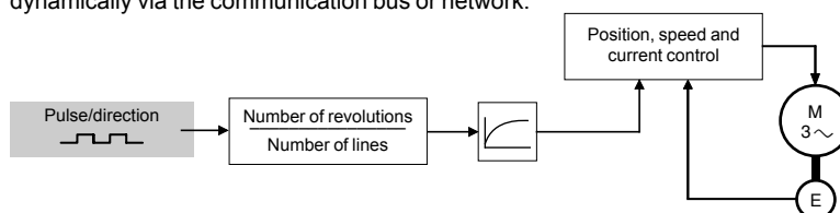
Electronic gearing mode
