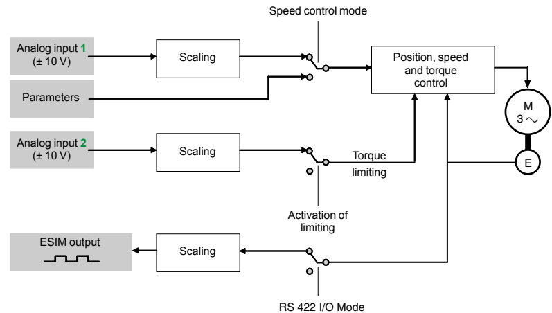
Instantaneous speed control operating mode
