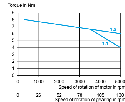
ILE1●661 with straight teeth gear G3
