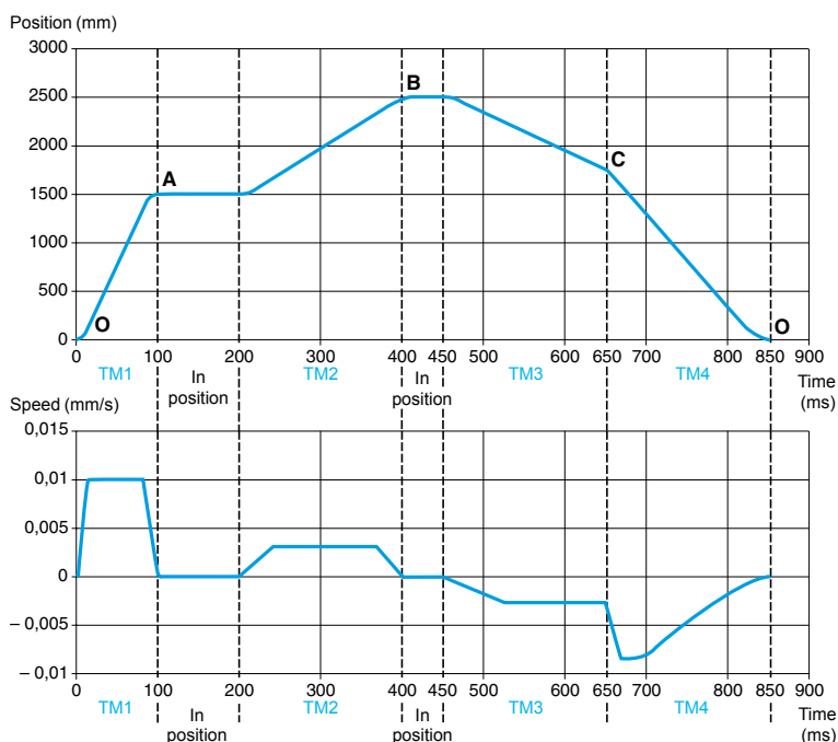
Example of a movement executed using 4 motion tasks
