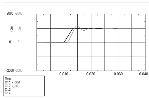
Oscilloscope function
