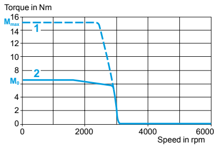
With LXM 15LD21M3 servo drive 230 V 3-phase
