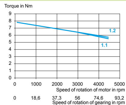
ILE2●661 with worm gear G7
