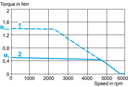
With LXM 05●D10F1 servo drive 115 V single-phase
