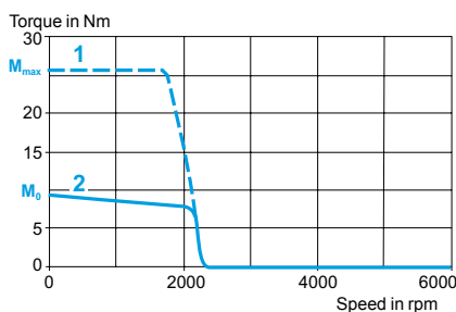
With LXM 15LD28M3 servo drive 230 V 3-phase
