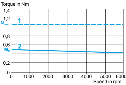
With LXM 05CU70M2 servo drive 230 V single-phase
