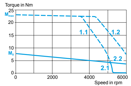
With LXM 15MD40N4 servo drive 400/480 V 3-phase
