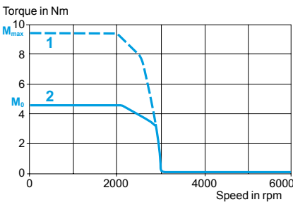
With LXM 15LD21M3 servo drive 230 V single-phase
