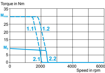
With LXM 15LD17N4 servo drive 400/480 V 3-phase
