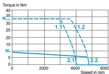
400/480 V 3-phase
