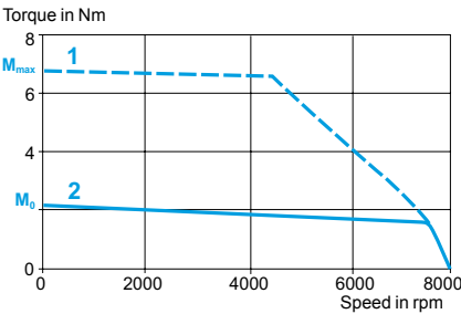
With LXM 05●D28M2 servo drive 230 V single-phase
