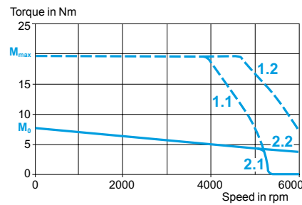
With LXM 15MD28N4 servo drive 400/480 V 3-phase
