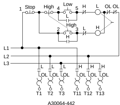
2-Speed Separate Winding Constant HP, Constant Torque and Variable Torque NEMA Size 0-4 Sizes 5, 6 & 7 Use Special Circuitry
