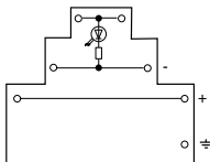
AB1ET3235UTLM (Resistance = 2.2 k \Omega , 0.35 W)
