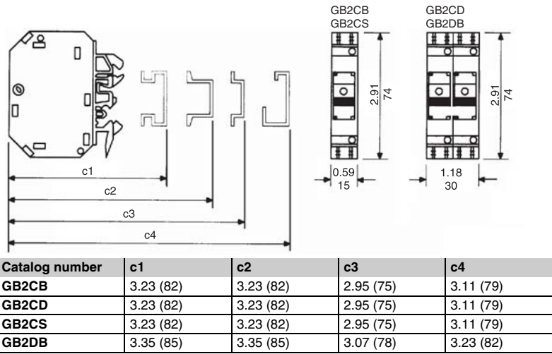
Approximate Dimensions, in. (mm)
