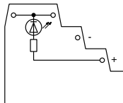
AB1DDP235TPL (Resistance = 2.2 k \Omega , 0.35 W)
