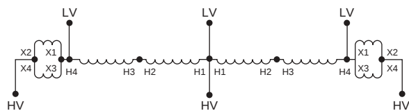
Wiring Diagram 5
