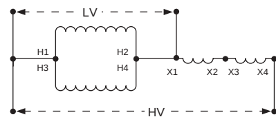
Wiring Diagram 2
