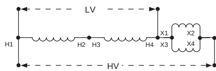
Wiring Diagram 3
