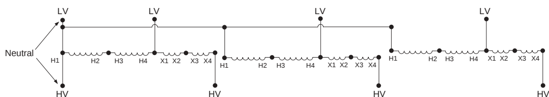
Wiring Diagram 10
