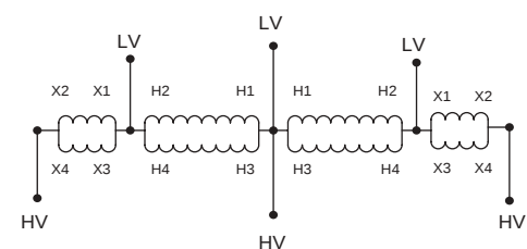
Wiring Diagram 11
