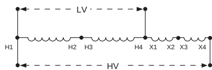
Wiring Diagram 4
