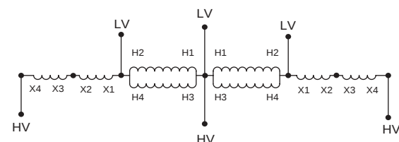
Wiring Diagram 12
