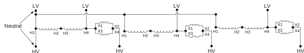
Wiring Diagram 9
