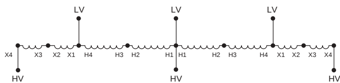
Wiring Diagram 6
