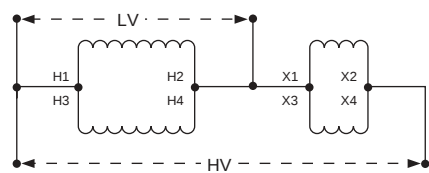
Wiring Diagram 1
