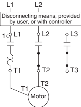
Figure 12: Three-phase starter wiring to control a single-phase motor
