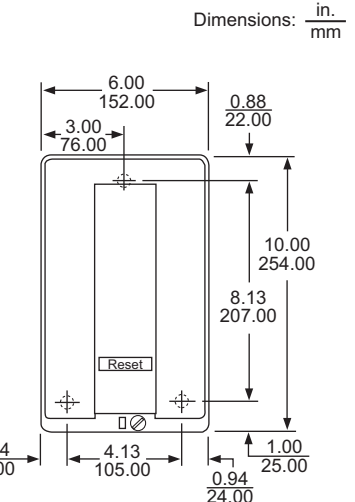
Type DPSG, 2 and 3 Pole 20-40 Full Load Amperes
