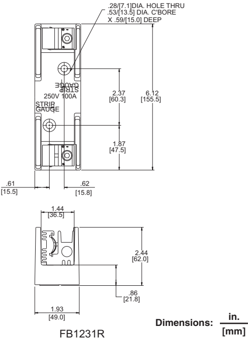
100 A, 250 V 9080FB Fuseholders
