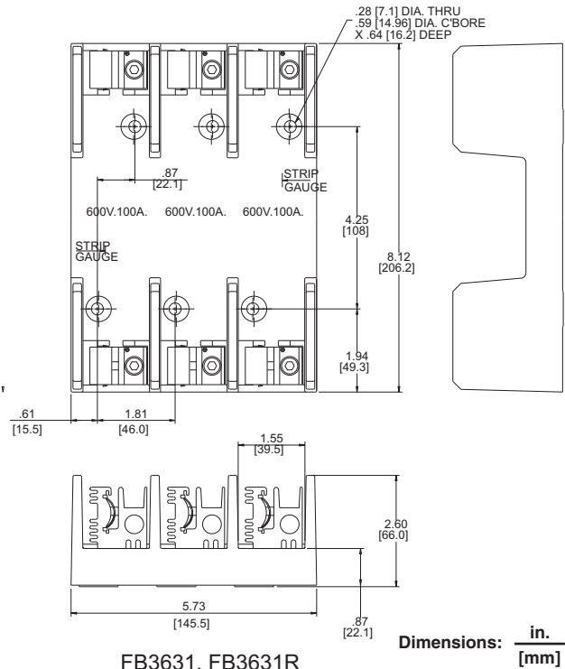
100 A, 250 V 9080FB Fuseholders
