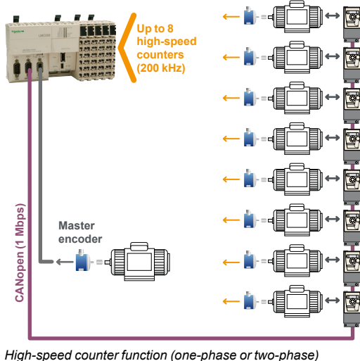
High-speed counter function (one-phase or two-phase)
