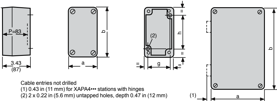
Undrilled Insulated enclosures XAPA1100, XAP2100
