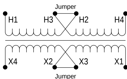
Series Connections
