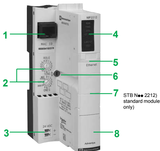
Interface modules with network/bus address selectors
