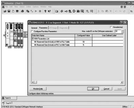
Configuring the exchange memory size with Advantys STB SPU 1 configuration software
