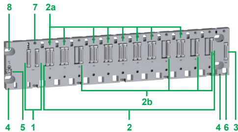
BMEXBP1200 backplane
