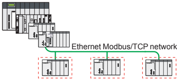
Ethernet Modbus/TCP network Ethernet Modbus/TCP DIO drop connected to an automation system platform
