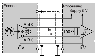
Wiring diagrams Type R (N) output stage
