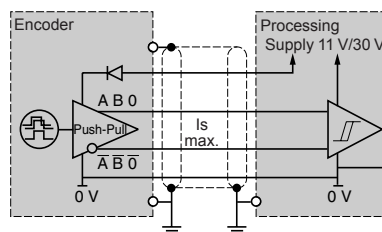
Type K (N) output stage
