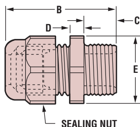
SEALING NUT
