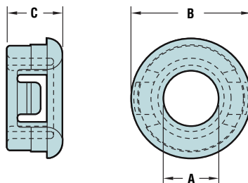
SINGLE PANEL THICKNESS
