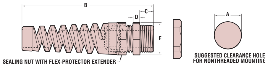
SEALING NUT WITH FLEX-PROTECTOR EXTENDER
