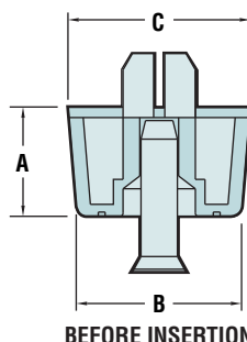
BEFORE INSERTION
