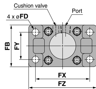
Head Side Flange
