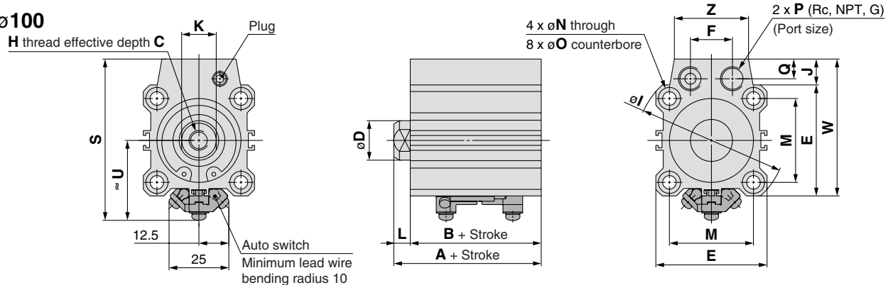
Rod End Male Thread (mm)
