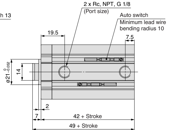
With boss on head end
