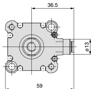
Built-in one-touch fittings: Ø32
