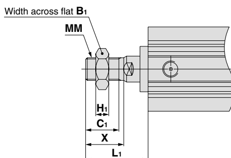
Rod end male thread
