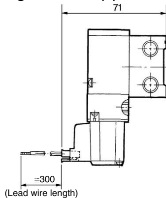
L plug connector (L)
