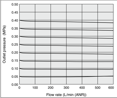
ARP30(K) Rc 3/8
