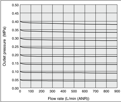
ARP40(K) Rc 1/2
