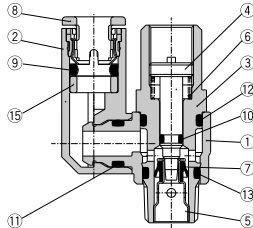
Universal type Meter-out type
