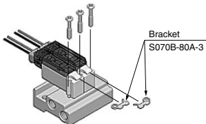
Manifold with 2 stations
