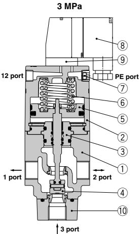
3-port valve (Dual pressure type)
