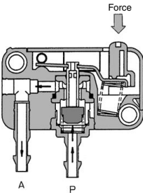
Bottom ported/Actuated
