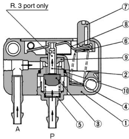
Bottom ported/Non-actuated
