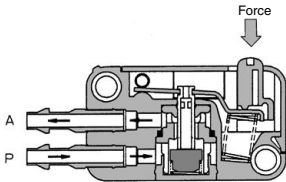
Side ported/Actuated
