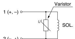
With surge voltage suppressor
