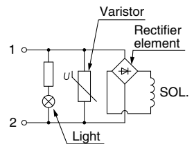
With light/surge voltage suppressor
