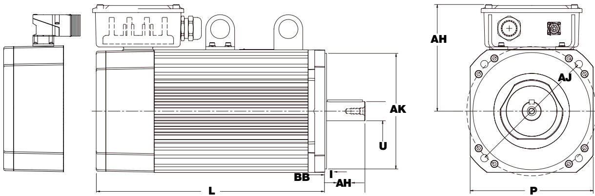
Rotatable Connector
