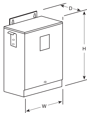
Encapsulated 1000 VA–10000 VA
