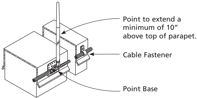
Typical Parapet Air Terminal
