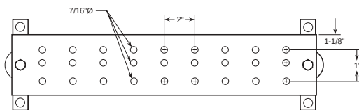
Ground Bar P/N EGBA14420CC (1/4 x 4 x 20")
