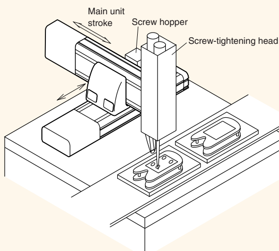
5–Screw-tightening machine in assembly line
