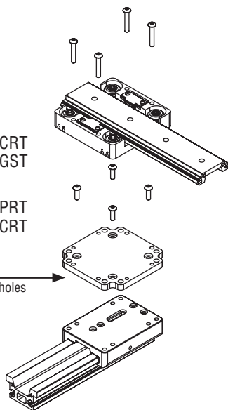
Two UGA (low profile) rails connected with the carriage mounting plate.
