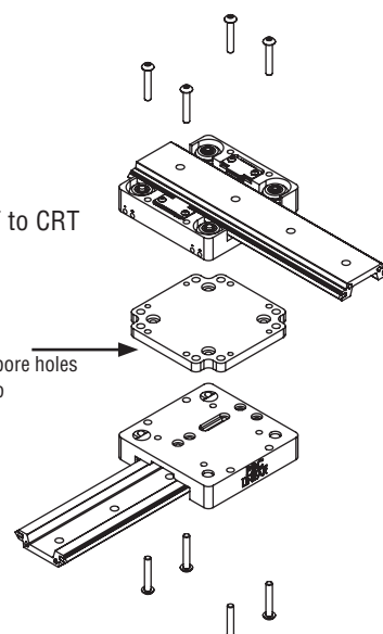
A combination—one UGT (tall) and one UGA (low profile) rail attached with the carriage mounting plate.
