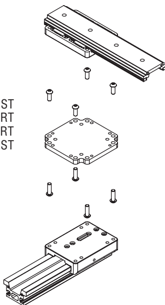
Two UGT (tall) rails connected with the carriage mounting plate.
