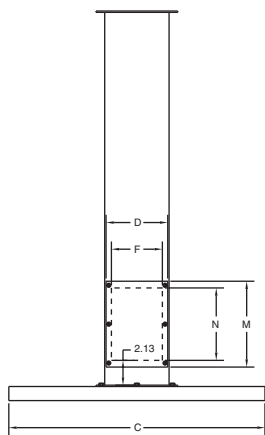
STRAIGHT PEDESTALS
