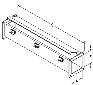
Straight Section
