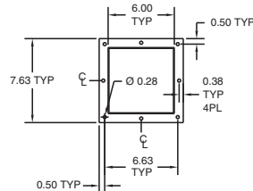
TOP AND BOTTOM FLANGES 6 X 6
