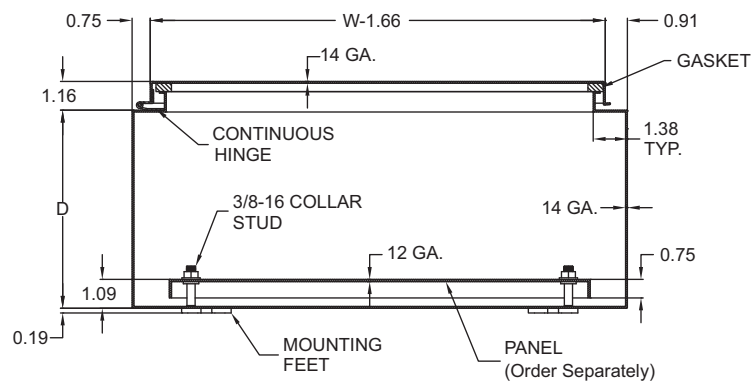
SECTION X-X
