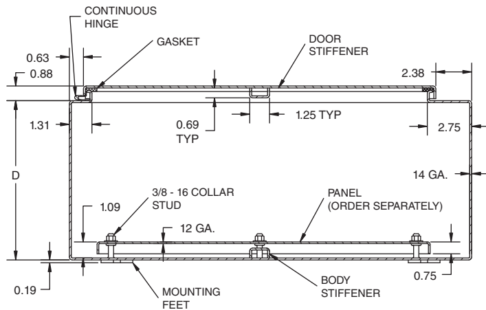
SECTION X-X
