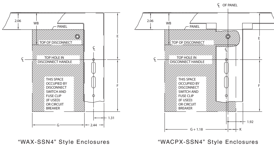
"WAX-SSN4" Style Enclosures
