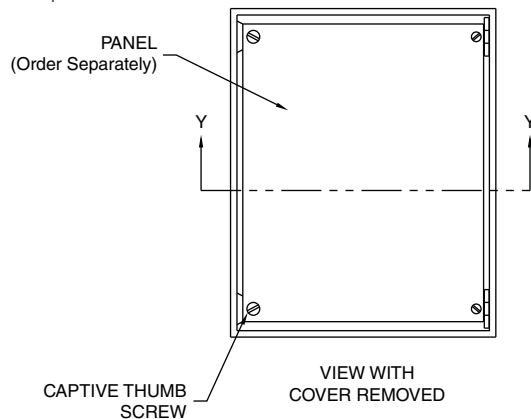
JIC Swing-Out Panel Kit
