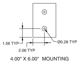
4.00" X 6.00" MOUNTING
