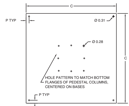
TOP VIEW OF BASES
