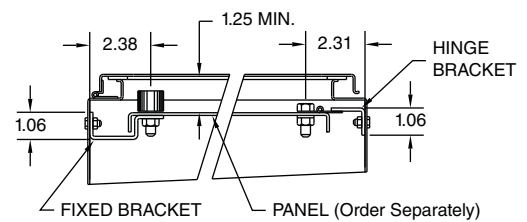
SECTION X-X
