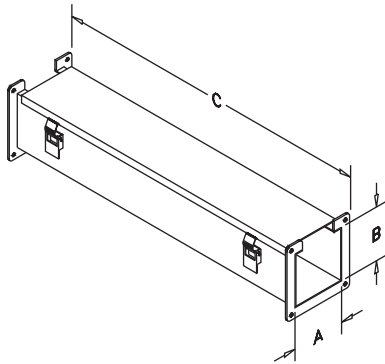
Straight
