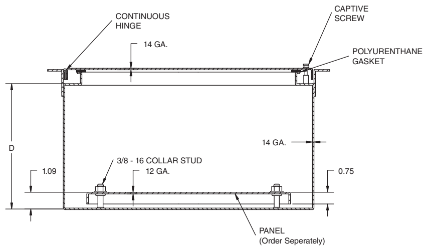
SECTION X-X
