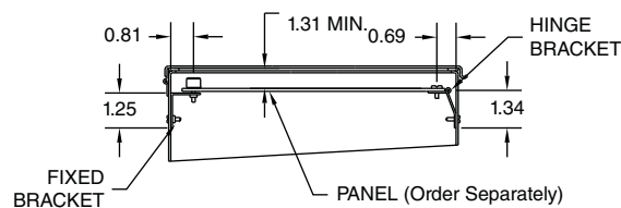
SECTION Y-Y
