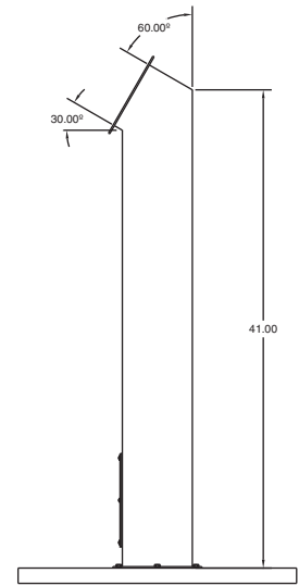
ANGLED PEDESTALS
