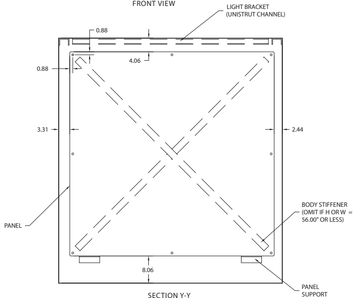
SECTION Y-Y
