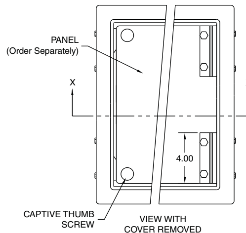
NEMA Swing-Out Panel Kit
