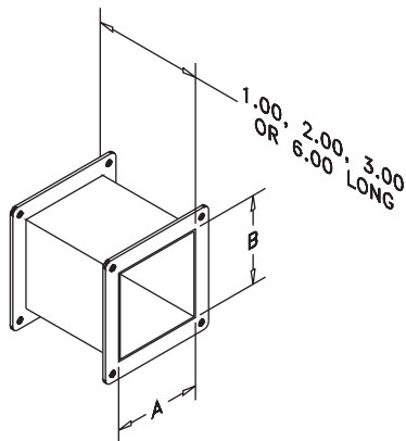
Nipple
