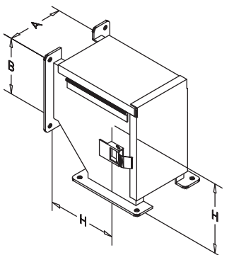
90° Elbow Outside Opening
