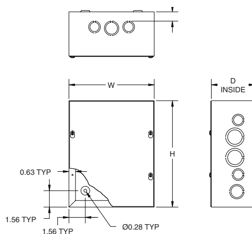
4.00" X 4.00" MOUNTING
