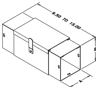
Telescope Fitting
