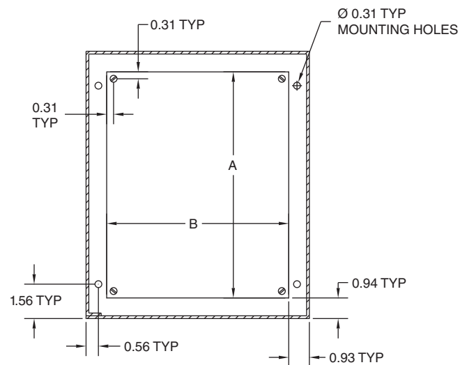
SECTION Y-Y
