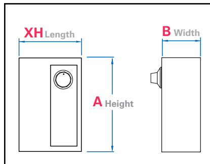
Enclosed Models
