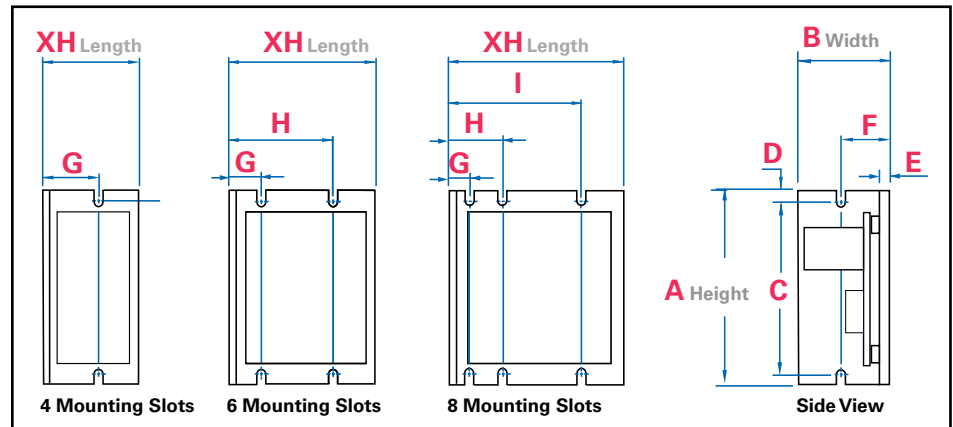
Chassis Models
