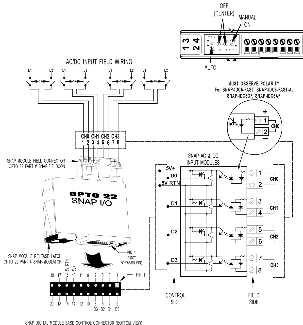
MA Modules with Manual/Auto Switches (Top View)
