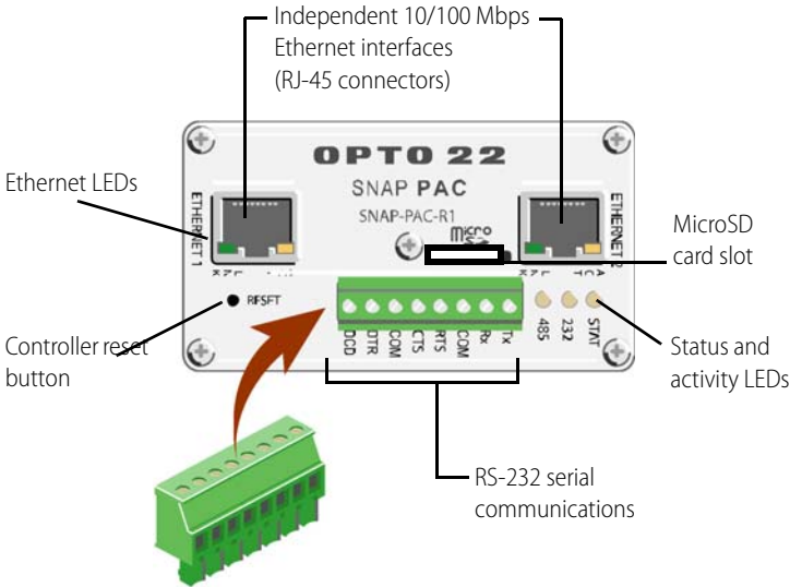
Status and Activity LEDs
