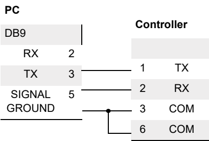
RS-232 Serial Cable Wiring*
