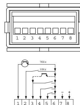
Slow count input (2) or reset input (3)
