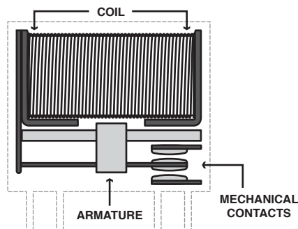
Typical Electromechanical PCB Relay
