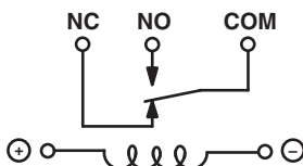
Figure T SPDT
