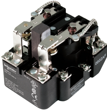
199 Series Relay
