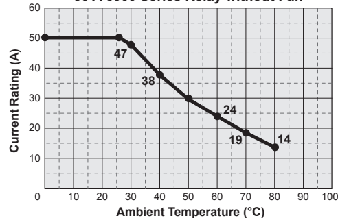
50 A 6000 Series Relay without Fan
