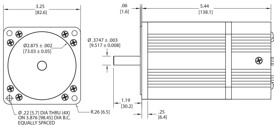
FRONT VIEW
