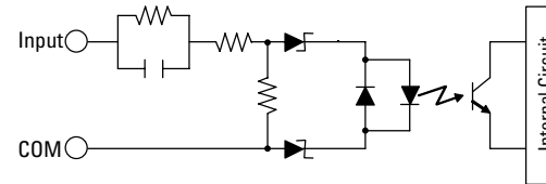
FC4A-N08A11
