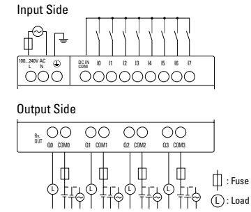
FT1A-※12RC
