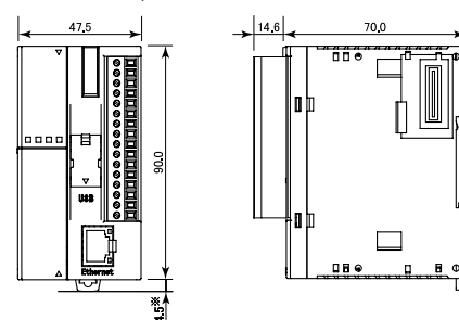
FC5A-D12K1E, FC5A-D12S1E
