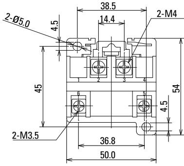
RL1N-D Screw Terminal 1 Pole DIN Rail Mount
