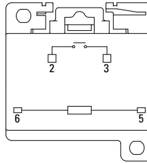
Screw Terminal 2 Pole DIN Rail Mount
