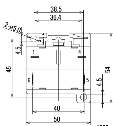
RL1B-D Quick Connect Terminal 1 Pole DIN Rail Mount
