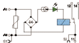
RB...121 A
