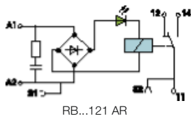
RB...121 AR
