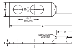
Figure 2: Slotted
