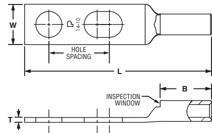
Figure 2: Slotted
