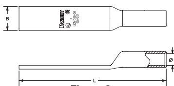
Figure 2. Blank Tongue
