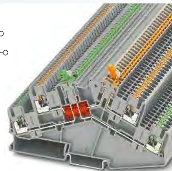
16 A, double-level terminal block with one disconnect knife per level, desk design
