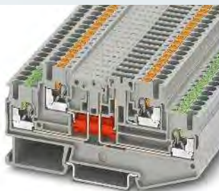
16 A, double-level terminal block, one disconnect zone
