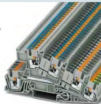
30 A, three-level terminal block, 1 x L outer conductor, 1 x N conductor, 1 x PE
