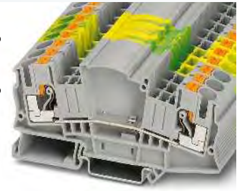
41 A, feed-through terminal block, same shape
