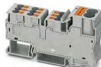
57 A, potential collective terminal block, 2 inputs 10 mm², 9 inputs 4 mm²
