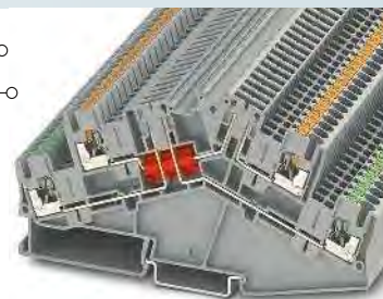
16 A, double-level terminal block, two disconnect zones
