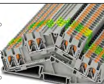
24 A, double-level terminal block, 4 connections per level
