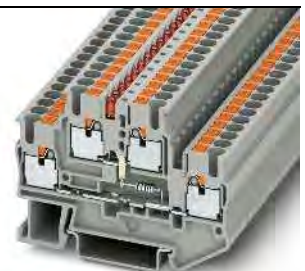
24 A, double-level terminal block with LED display
