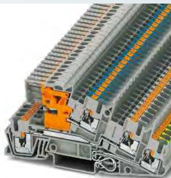
30 A, three-level terminal block, 1 x L outer conductor, 1 x N conductor can be disconnected, 1 x PE
