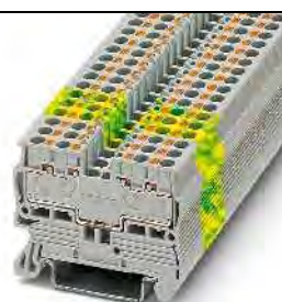
24 A, feed-through terminal block, 4 connections
