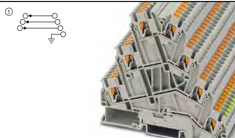
25 A, four-level terminal block with PE foot
