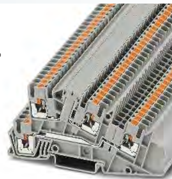
30 A, three-level terminal block, 2 x L outer conductors
