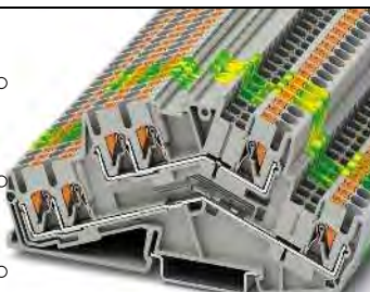
24 A, double-level terminal block, 3 connections per level
